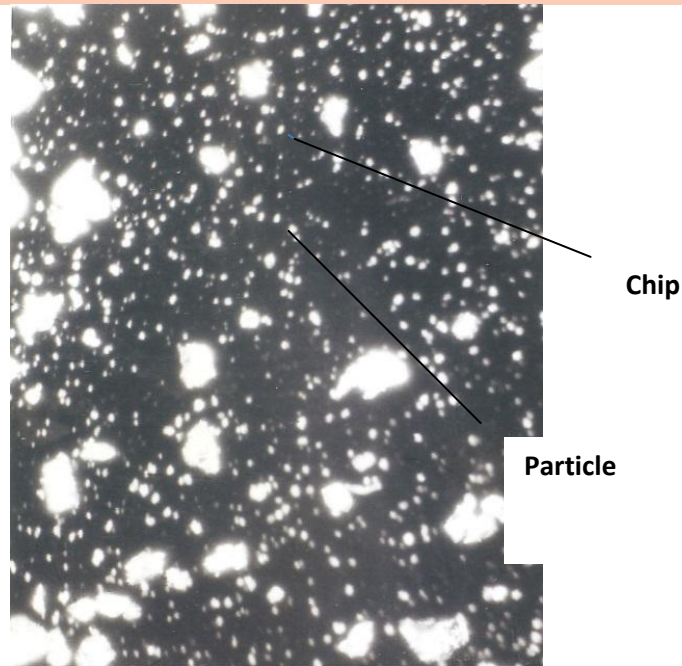
FIGURE 2. Optical micrograph , (X1000), of the Silver –Tin alloy manufactured by quenching method and before annealing .
