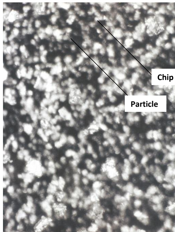
FIGURE 3. Optical micrograph , (X1000), of the Silver –Tin alloy manufactured by quenching method after annealing at 400 C 0 .
