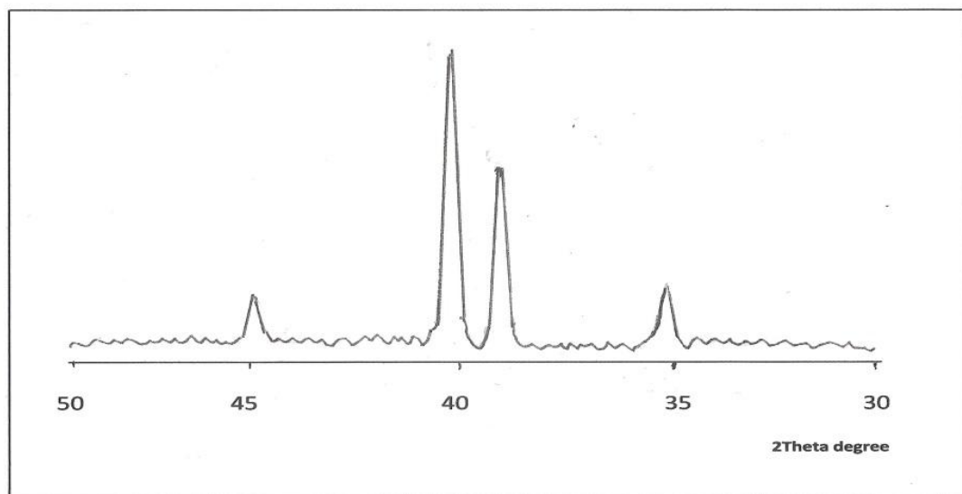
FIGURE 1 . X-ray diffraction pattern for the Silver – Tin Amalgam alloy , manufactured by rapid quenching method , \gamma - (Ag 3 Sn at 2\theta^0 = 35 , 38,40 respectively ) and \epsilon - ( Cu 3 Sn at 2\theta^0 = 44 ) .
